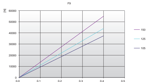
Load / Elongation [ % ]
